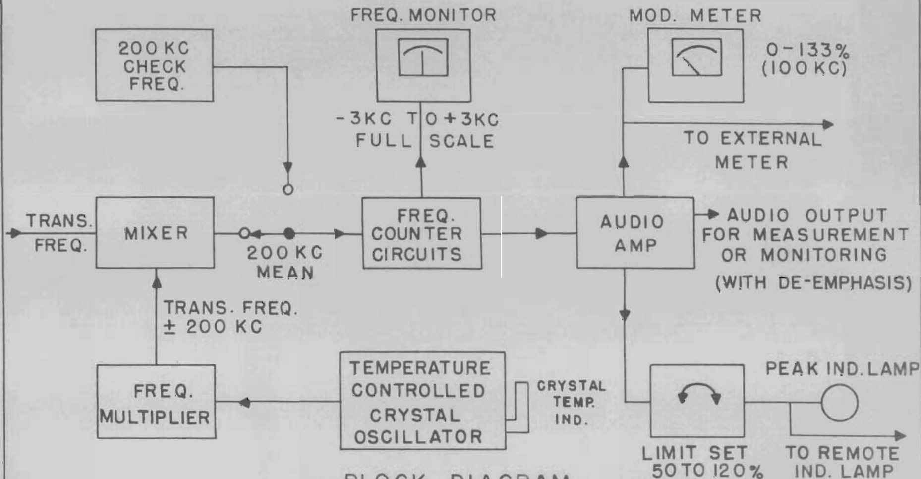
BLOCK DIAGRAM
